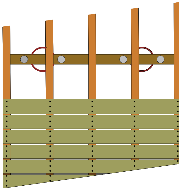
SECTION VIEW
